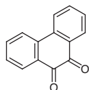
9,10-Phenanthrenequinone CAS RN: 84-11-7
