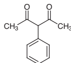
3-Phenylacetylacetone CAS RN: 5910-25-8
