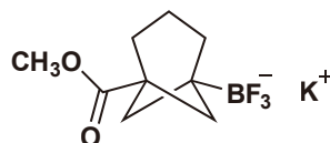
Potassium Trifluoro- [5-(methoxycarbonyl)- bicyclo[3.1.1]heptan- 1-yl]borate
