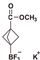
Potassium Trifluoro- [3-(methoxycarbonyl)- bicyclo[1.1.1]pentan- 1-yl]borate
