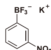
Potassium (3-Nitrophenyl)trifluoroborate 1g [P1819]
