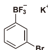
Potassium (3-Bromophenyl)trifluoroborate 1g / 5g [P2646]
