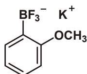
Potassium (2-Methoxyphenyl)trifluoroborate 1g / 5g [P1810]
