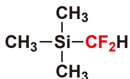
(Difluoromethyl)trimethylsilane
