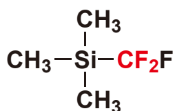
Ruppert-Prakash Reagent
