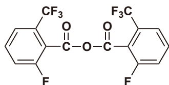
2-Fluoro-6-(trifluoromethyl)-benzoic Anhydride (= FTFBA)
