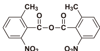
2-Methyl-6-nitrobenzoic Anhydride (= MNBA)
