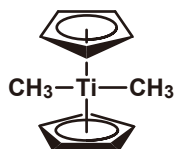
Dimethyltitanocene
