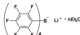
Lithium Tetrakis(pentafluorophenyl)borate - Ethyl Ether Complex
