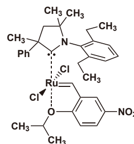
UltraNitroCat 100mg [U0116]
