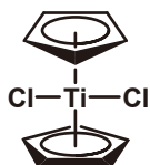
Titanocene Dichloride
