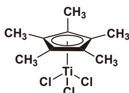
(Pentamethylcyclopentadienyl)titanium(IV) Trichloride
