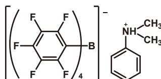
N,N-Dimethylanilinium Tetrakis(pentafluorophenyl)borate
