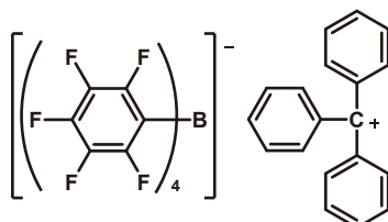
Triphenylmethylm Tetrakis(pentafluorophenyl)borate
