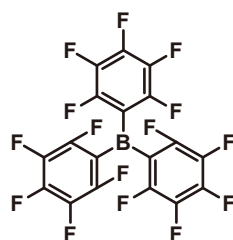
Tris(pentafluorophenyl)borane
