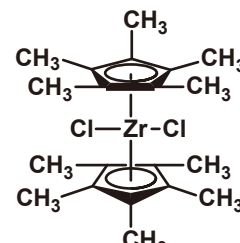
Decamethylzirconocene Dichloride
