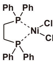
[1,2-Bis(diphenylphosphino)ethane]nickel(II) Dichloride
