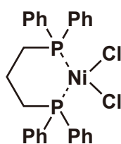
[1,3-Bis(diphenylphosphino)propane]nickel(II) Dichloride
