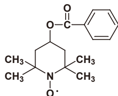
4-Hydroxy-TEMPO Benzoate Free Radical
