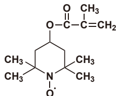
4-Methacryloyloxy-TEMPO Free Radical
