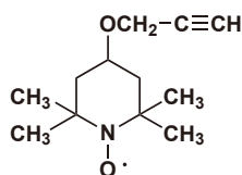
4-Propargyloxy-TEMPO Free Radical
