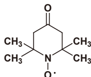
4-Oxo-TEMPO Free Radical
