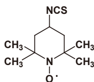
4-Isothiocyanato-TEMPO Free Radical
