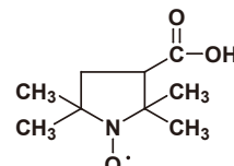
3-Carboxy-PROXYL Free Radical
