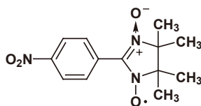
p-NPNN Free Radical
