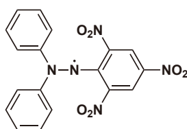
DPPH Free Radical
