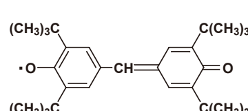
Galvinoxyl Free Radical
