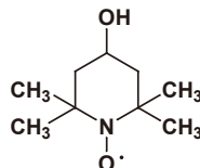
4-Hydroxy-TEMPO Free Radical
