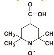
4-Carboxy-TEMPO Free Radical
