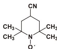
4-Cyano-TEMPO Free Radical
