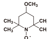
4-Methoxy-TEMPO Free Radical
