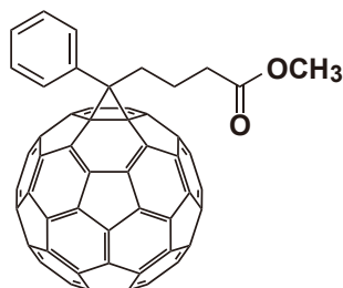
[60]PCBM
