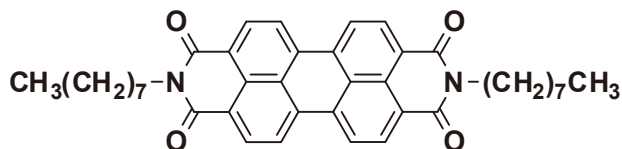
N,N'-Di-n-octyl-3,4,9,10-perylene-tetracarboxylic Diimide
