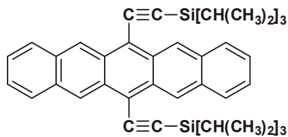
TIPS Pentacene
