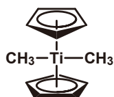
Dimethyltitanocene
