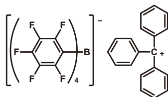
Triphenylmethylium Tetrakis(pentafluorophenyl)borate
