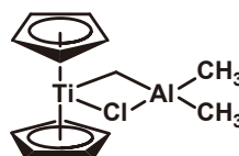
Tebbe Reagent
