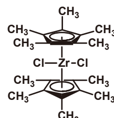
Decamethylzirconocene Dichloride
