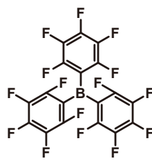
Tris(pentafluorophenyl)borane
