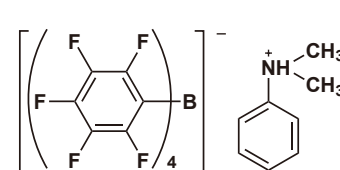
N,N-Dimethylanilinium Tetrakis(pentafluorophenyl)borate
