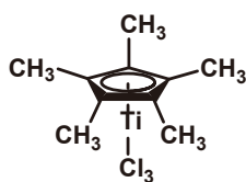
(Pentamethylcyclopentadienyl)-titanium(IV) Trichloride
