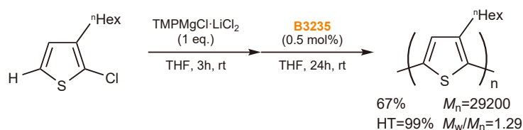
[1,3-Bis(2,6-diisopropylphenyl)imidazol-2-ylidene]triphenylphosphine Nickel(II) Dichloride
