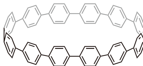
[12]Cycloparaphenylene 10mg [C2449]
