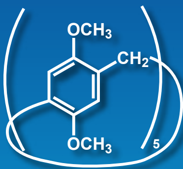
Dimethoxypillar[5]arene
