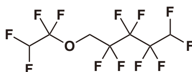
1H,1H,5H-Octafluoropentyl 1,1,2,2-Tetrafluoroethyl Ether
