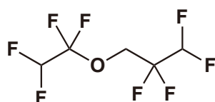
1,1,2,2-Tetrafluoroethyl 2,2,3,3-Tetrafluoroethyl Ether
