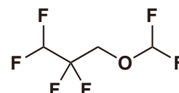
Difluoromethyl 2,2,3,3-Tetrafluoropropyl Ether
