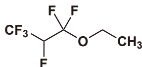
Ethyl 1,1,2,3,3,3-Hexafluoropropyl Ether
