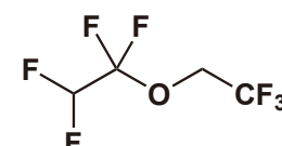
1,1,2,2-Tetrafluoroethyl 2,2,2-Trifluoroethyl Ether
