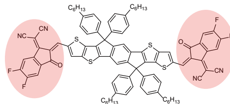
IT4F: PCE = 13.1% 2)
