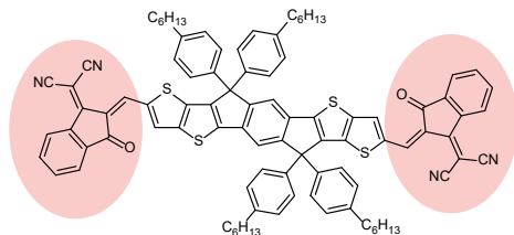
ITIC: PCE = 11.2% 1)
