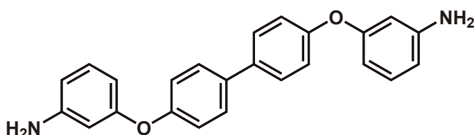
43BAPOBP
