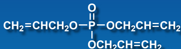
Triallyl Phosphate
