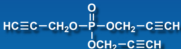
Tripropargyl Phosphate
