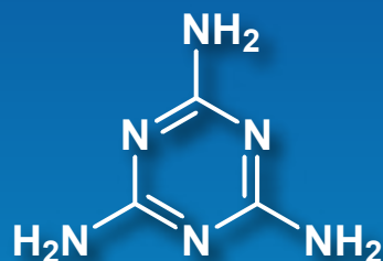
Melamine Monomer
