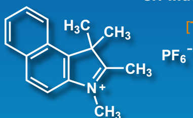
1,1,2,3-Tetramethyl-1H-benzo[e]indolium Hexafluorophosphate 5g / 25g [T3457]
