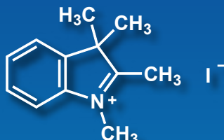
1,2,3,3-Tetramethyl-3H-indolium iodide 5g [T3979] New
