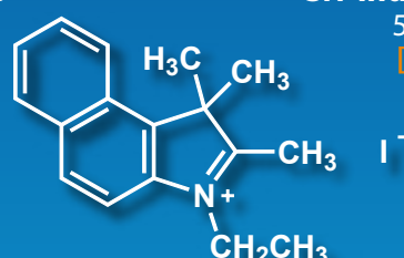
3-Ethyl-1,1,2-trimethyl-1H-benzo[e]indolium iodide 5g / 25g [E1545] New
