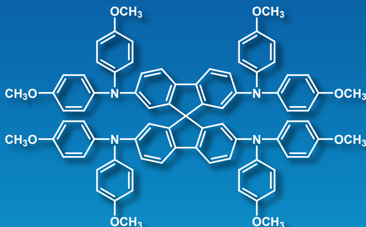
Spiro-OMeTAD
