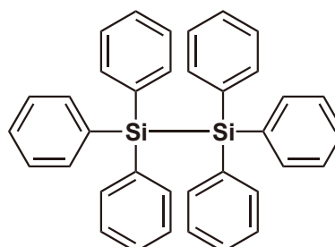
Hexaphenyldisilane 1g / 5g [H0119]
