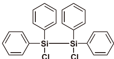
1,2-Dichloro-1,1,2,2-tetraphenyldisilane 1g / 5g [D6052] New
