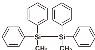
1,2-Dimethyl-1,1,2,2-tetraphenyldisilane 5g [D5031]
