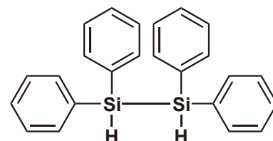
1,1,2,2-Tetraphenyldisilane 1g / 5g [T1896]
