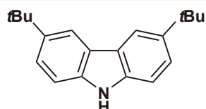
3,6-Di-tert-butylcarbazole
