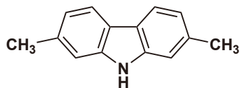
2,7-Dimethyl-9H-carbazole
