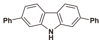
2,7-Diphenyl-9H-carbazole
