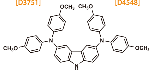
3,6-Bis[N,N-bis(4-methoxyphenyl)amino]-9H-carbazole
