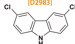
3,6-Dichlorocarbazole
