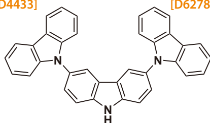
9,3':6',9''-Tercarbazole
