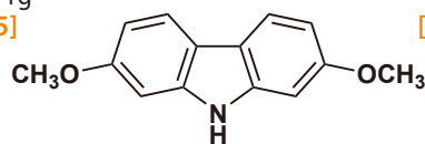
2,7-Dimethoxy-9H-carbazole
