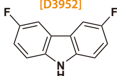
3,6-Difluoro-9H-carbazole
