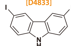
3,6-Diiodocarbazole
