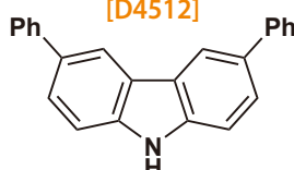
3,6-Diphenylcarbazole
