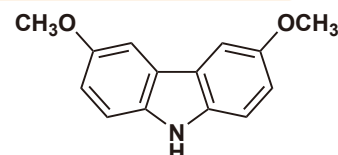
3,6-Dimethoxy-9H-carbazole
