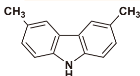
3,6-Dimethylcarbazole
