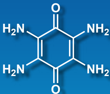
2,3,5,6-Tetraamino-1,4-benzoquinone (= TABQ) 1g / 5g [T4344]
