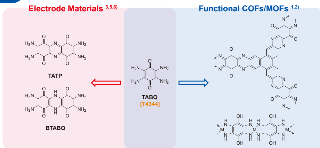
2,3,5,6-Tetraamino-1,4-benzoquinone (= TABQ) 1g / 5g [T4344]
