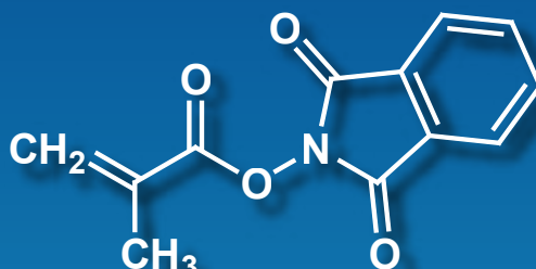
N-Phthalimidyl Methacrylate
