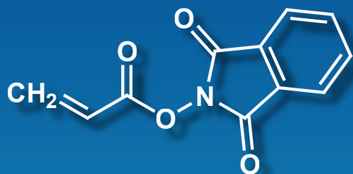
N-Phthalimidyl Acrylate
