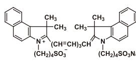
Indocyanine Green
