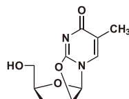
2,2'-O-Anhydro-5-methyluridine
