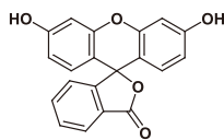
Fluorescein
