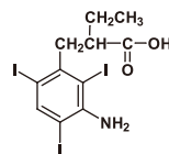
Iopanoic acid
