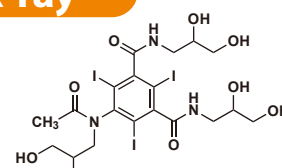
Iohexol (mixture of isomers) 5g / 25g [I0903]
