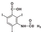
Acetrizic Acid 1g / 5g [A0858]
