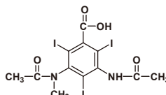
Metrizic Acid 5g / 25g [M1363]
