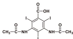
Diatrizic Acid 25g [D1462]
