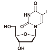
2'-Deoxy-5-fluorouridine 100mg / 500mg / 1g [D2235]
