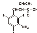
Iopanoic Acid 5g / 25g [I0300]
