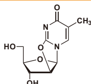
2,2'-O-Anhydro-5-methyluridine 1g [A2431]
