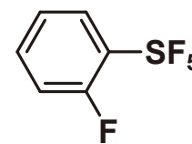
2-Fluorophenylsulfur Pentafluoride
