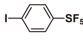
4-Iodophenylsulfur Pentafluoride
