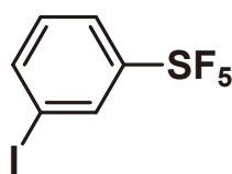
3-Iodophenylsulfur Pentafluoride
