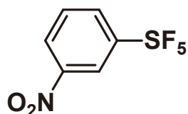
3-Nitrophenylsulfur Pentafluoride
