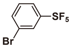
3-Bromophenylsulfur Pentafluoride
