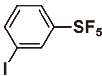
3-Iodophenylsulfur Pentafluoride
