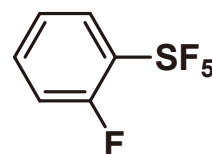
2-Fluorophenylsulfur Pentafluoride
