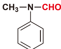
N-Methylformanilide
