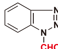
1H-Benzotriazole-1-carboxaldehyde
