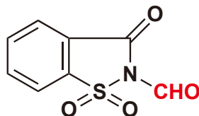
N-Formylsaccharin
