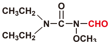
N-(Diethylcarbamoyl)- N-methoxyformamide
