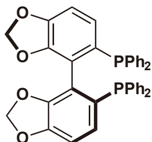
(S)-(-)-SEGPHOS®
