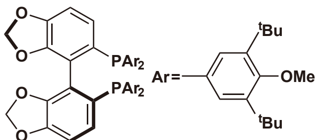
(S)-(+)-DTBM-SEGPHOS®
