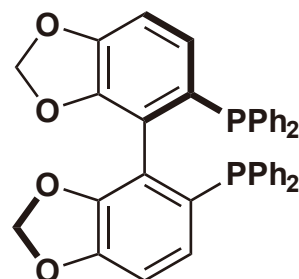
(R)-(+)-SEGPHOS®
