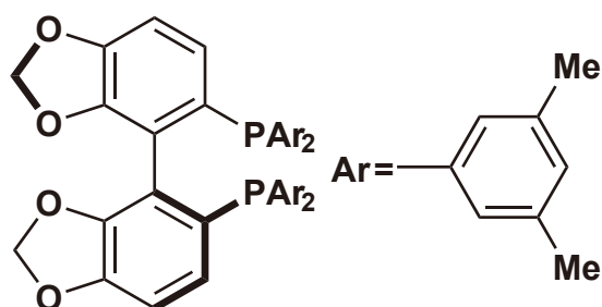
(S)-(-)-DM-SEGPHOS®
