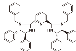
PyBidine
