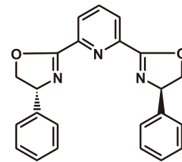
( R,R )-2,6-Bis(4-phenyl-2-oxazolin-2-yl)pyridine
