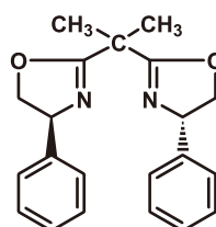
( S,S )-2,2-Bis(4-phenyl-2-oxazolin-2-yl)propane
