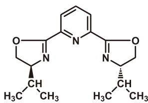
( S,S )-2,6-Bis(4-isopropyl-2-oxazolin-2-yl)pyridine
