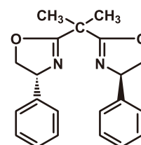
( R,R )-2,2-Bis(4-phenyl-2-oxazolin-2-yl)propane
