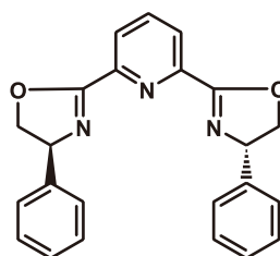
( S,S )-2,6-Bis(4-phenyl-2-oxazolin-2-yl)pyridine
