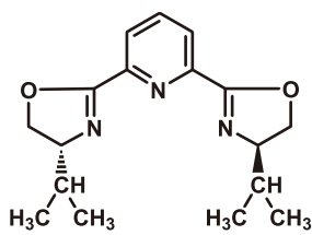
( R,R )-2,6-Bis(4-isopropyl-2-oxazolin-2-yl)pyridine
