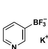
Potassium 3-Pyridyltrifluoroborate
