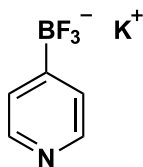
Potassium 4-Pyridyltrifluoroborate
