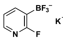
Potassium Trifluoro(2-fluoropyridin- 3-yl)borate
