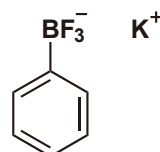
Potassium Phenyltrifluoroborate
