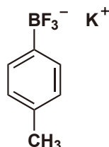
Potassium p-Tolyltrifluoroborate
