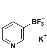
Potassium 3-Pyridyltrifluoroborate
