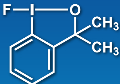
1-Fluoro-3,3-dimethyl-1,2-benziodoxole
