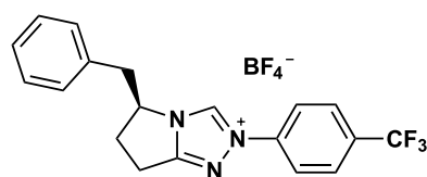
(S)-Benzyl-2-[4-(trifluoromethyl)phenyl]- 6,7-dihydro-5H-pyrrolo[2,1-c][1,2,4]- triazolium Tetrafluoroborate
