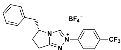
(R)-Benzyl-2-[4-(trifluoromethyl)phenyl]- 6,7-dihydro-5H-pyrrolo[2,1-c][1,2,4]- triazolium Tetrafluoroborate
