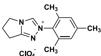
6,7-Dihydro-2-(2,4,6-trimethylphenyl)-5H-pyrrolo[2,1-c]-1,2,4-triazolium Perchlorate
