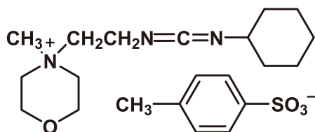
1-Cyclohexyl-3-(2-morpholinoethyl)-carbodiimide Metho- p -toluenesulfonate (CMC)
