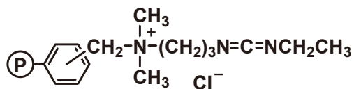
1-(3-Dimethylaminopropyl)-3-ethylcarbodiimide Resin cross-linked with 1% DVB (50-100mesh) (1.0-1.3mmol/g) (PS-EDC)
