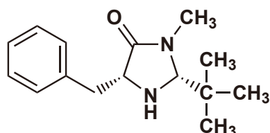
(2R,5R)-(+)-2-tert-Butyl-3-methyl-5-benzyl-4-imidazolidinone
