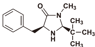
(2S,5S)-(-)-2-tert-Butyl-3-methyl-5-benzyl-4-imidazolidinone
