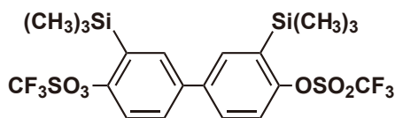
3,3'-Bis(trimethylsilyl)- biphenyl-4,4'-diyl Bis(trifluoromethanesulfonate) 1g [B3047]
