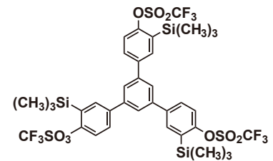
1,3,5-Tris[4- (trifluoromethanesulfonyloxy)- 3-(trimethylsilyl)phenyl]benzene 1g 33,700円 [T2467]
