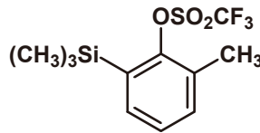
2-Methyl- 6-(trimethylsilyl)phenyl Trifluoromethanesulfonate 1g 18,600円 / 5g 64,200円 [M1883]
