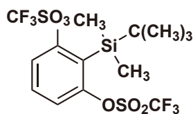
2-(tert-Butyldimethylsilyl)- 1,3-phenylene Bis(trifluoromethanesulfonate)
