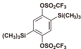
2,5-Bis(trimethylsilyl)- 1,4-phenylene Bis(trifluoromethanesulfonate)
