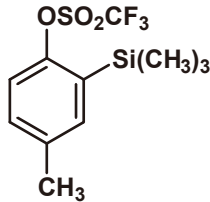
4-Methyl- 2-(trimethylsilyl)phenyl Trifluoromethanesulfonate 1g 16,300円 / 5g 56,000円 [M1882]
