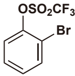
2-Bromophenyl Trifluoromethanesulfonate 5g 30,600円 [B4777]
