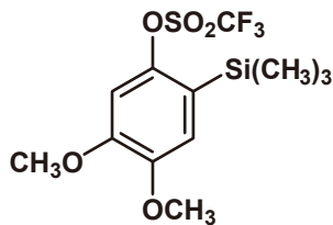
4,5-Dimethoxy- 2-(trimethylsilyl)phenyl Trifluoromethanesulfonate 1g 19,700円 / 5g 68,100円 [D3883]
