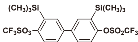
3,3'-Bis(trimethylsilyl)- biphenyl-4,4'-diyl Bis(trifluoromethanesulfonate) 1g 31,600円 [B3047]
