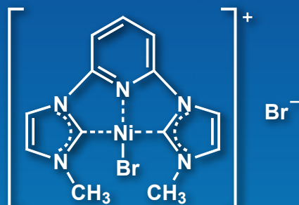
Bromo[(2,6-pyridinediyl)bis(3-methyl-1-imidazolyl-2-ylidene)]nickel Bromide
