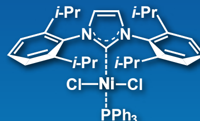
[1,3-Bis(2,6-diisopropylphenyl)imidazol-2-ylidene]triphenylphosphine Nickel(II) Dichloride
