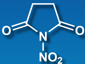
N-Nitrosuccinimide
