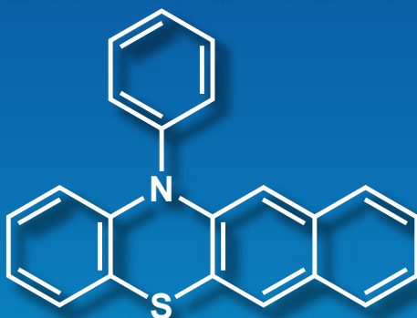
12-Phenyl-12H-benzo[b]phenothiazine
