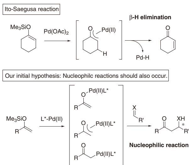
Scheme 2. Our original hypothesis.
