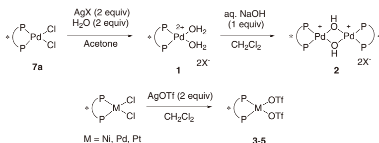
Scheme 3. Preparation of chiral metal complexes.
