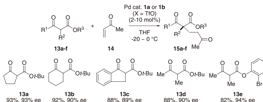
Scheme 8. Catalytic asymmetric Michael reaction of \beta -ketoesters.
