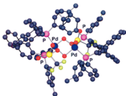
Pd- \mu -hydroxo complex
