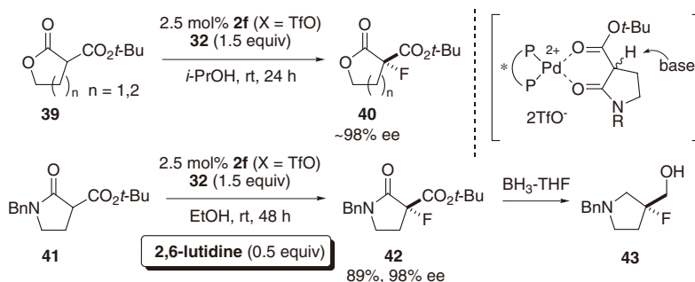
Scheme 16. Reactions of other related compounds.
