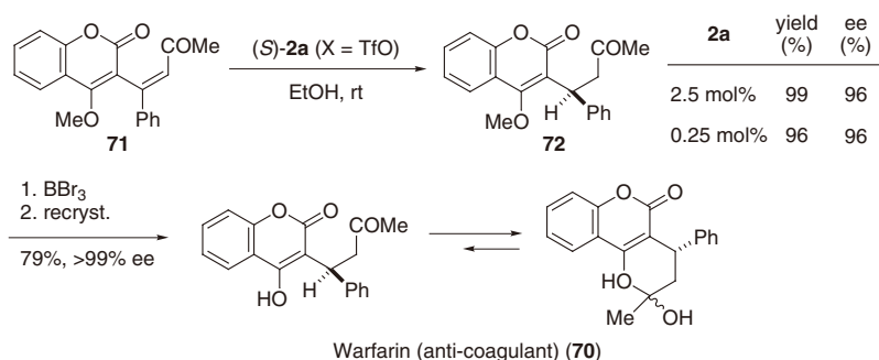
Scheme 24. Catalytic asymmetric synthesis of ( S )-warfarin.
