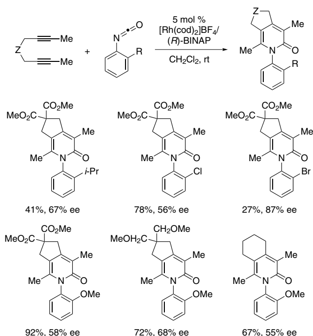
Scheme 17. Rhodium-catalyzed atroposelective [2+2+2] cycloaddition of diynes with aryl isocyanates
