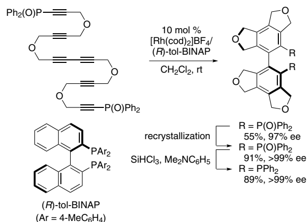
Scheme 15. Enantioselective synthesis of an axially chiral biaryl bisphosphine via the rhodium-catalyzed [2+2+2] cycloaddition of a hexayne
