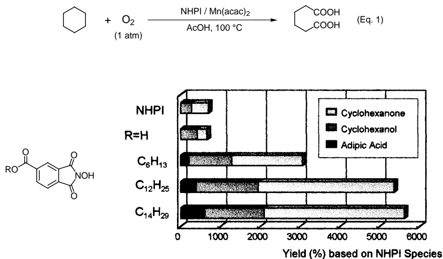
Figure 2. Oxidation of cyclohexane catalyzed by NHPI derivatives without solvent
