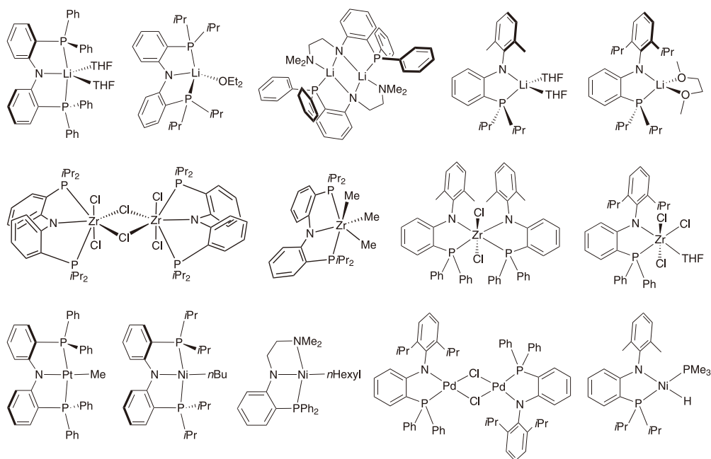
Figure 2. Representative examples of anilido phosphine complexes
