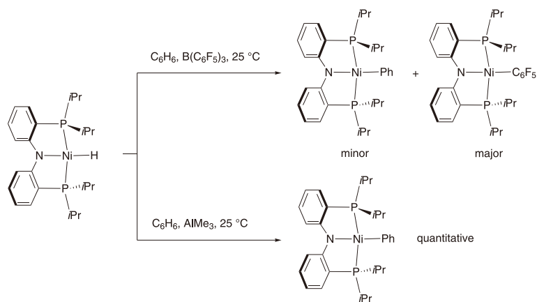
Scheme 3. Benzene C-H activation by [1b]NiH
