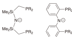
Figure 1. Representative amido phosphine ligands featuring distinct bridging backbones
