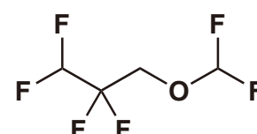
Difluoromethyl 2,2,3,3-Tetrafluoropropyl Ether
