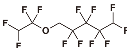
1H,1H,5H-Octafluoropentyl 1,1,2,2-Tetrafluoroethyl Ether
