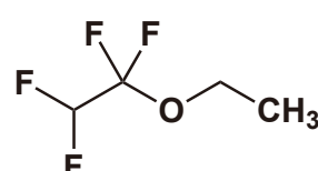
Ethyl 1,1,2,2-Tetrafluoroethyl Ether
