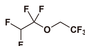
1,1,2,2-Tetrafluoroethyl 2,2,2-Trifluoroethyl Ether
