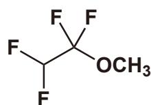
Methyl 1,1,2,2-Tetrafluoroethyl Ether
