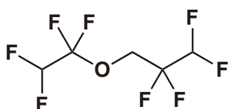
1,1,2,2-Tetrafluoroethyl 2,2,3,3-Tetrafluoropropyl Ether
