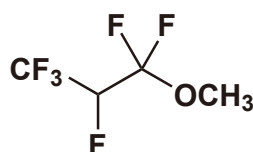
1,1,2,3,3,3-Hexafluoropropyl Methyl Ether
