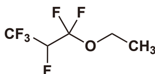
Ethyl 1,1,2,3,3,3-Hexafluoropropyl Ether
