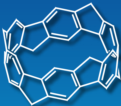
Methylene-bridged [6]cycloparaphenylene
