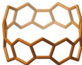
Methylene-bridged [6]CPP
