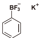
Potassium Phenyltrifluoroborate
