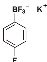
Potassium (4-Fluorophenyl)- trifluoroborate
