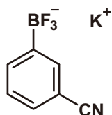
Potassium (3-Cyanophenyl)- trifluoroborate
