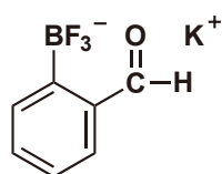
Potassium (2-Formylphenyl)- trifluoroborate
