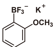
Potassium (2-Methoxyphenyl)- trifluoroborate
