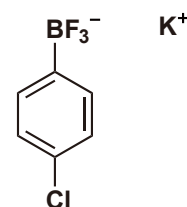
Potassium (4-Chlorophenyl)- trifluoroborate
