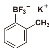
Potassium o-Tolyltrifluoroborate
