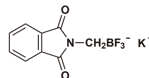
Potassium (Phthalimidomethyl)- trifluoroborate
