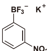
Potassium (3-Nitrophenyl)- trifluoroborate
