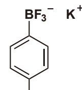
Potassium (4-Methoxyphenyl)- trifluoroborate
