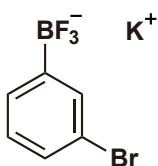
Potassium (3-Bromophenyl)- trifluoroborate
