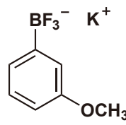
Potassium (3-Methoxyphenyl)- trifluoroborate
