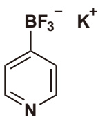
Potassium 4-Pyridyltrifluoroborate
