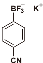
Potassium (4-Cyanophenyl)- trifluoroborate
