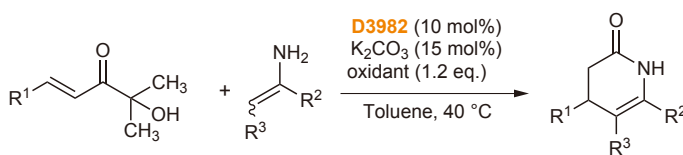
6,7-Dihydro-2-(2,4,6-trimethylphenyl)-5H-pyrrolo[2,1-c][1,2,4]triazolium Perchlorate
