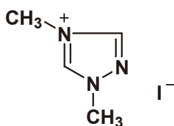
1,4-Dimethyl-1,2,4-triazolium Iodide
